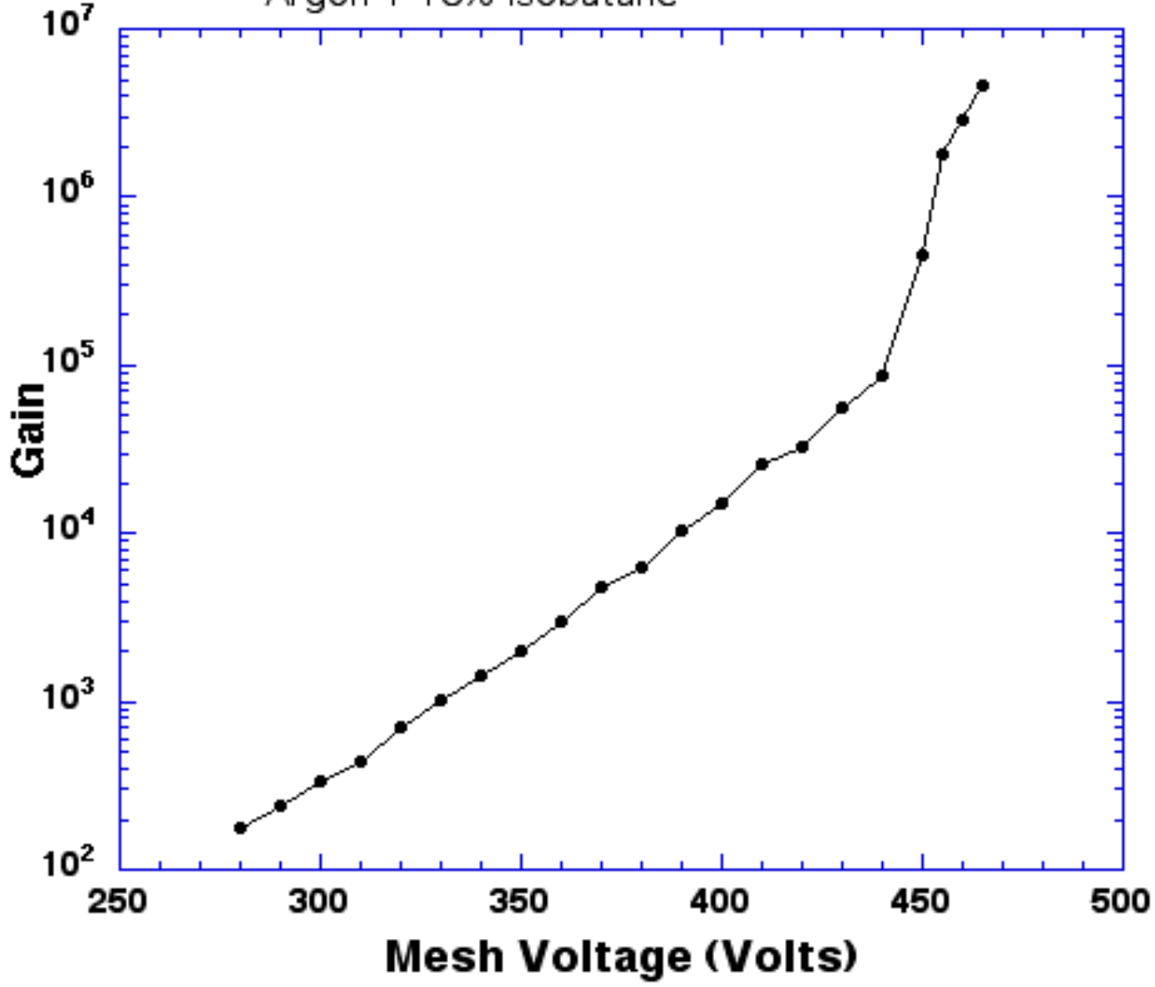
Micromegas (50 micron gap) with resistive foil Argon + 10% Isobutane
