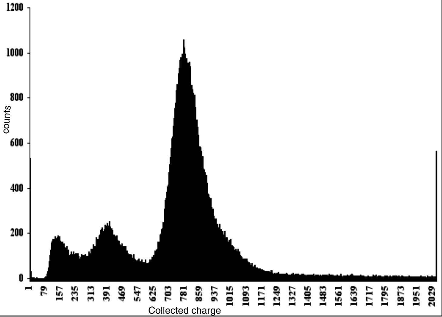
55Fe, Argon + 10% Isobutane, gain=6000
