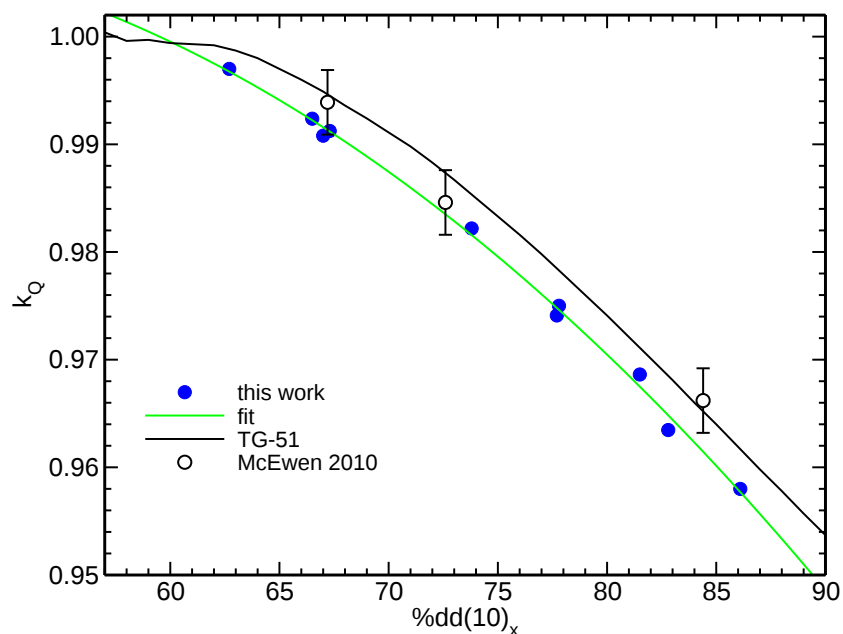
Figure 5: Monte Carlo calculated k_Q factors for the Exradin A12S ion chamber ( a, 0.25 \text{ cm}^3 ) along with measurements from McEwen 5 and TG-51 values. 6 The fit is to our Monte Carlo values.
