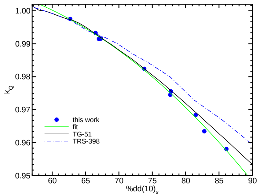
Figure 15: Monte Carlo calculated k_Q factors for the PTW30011 ion chamber ( d, 0.6 \text{ cm}^3 ) along with TRS-398 and TG-51 protocol values. 6,7 The fit is to our Monte Carlo values.
