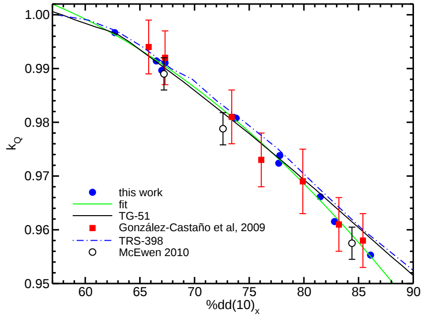
Figure 17: Monte Carlo calculated k_Q factors for the PTW30013 ion chamber ( e, 0.6 \text{ cm}^3 ) along with measurements from McEwen, 5 TRS-398 and TG-51 values 6,7 and Monte Carlo data from González-Castaño 8 et al. The fit is to our Monte Carlo values.
