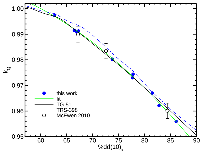
Figure 23: Monte Carlo calculated k_Q factors for the IBA FC65P ion chamber ( f, 0.65 \text{ cm}^3 ) along with measurements from McEwen, 5 TG-51 6 and TRS-398 values. 7 The fit is to our Monte Carlo values.
