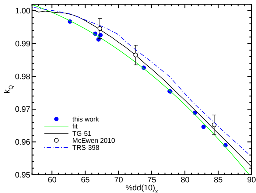
Figure 24: Monte Carlo calculated k_Q factors for the IBA CC25 ion chamber ( a, 0.25 \text{ cm}^3 ) along with measurements from McEwen, 5 TG-51 6 and TRS-398 values. 7 The fit is to our Monte Carlo values.
