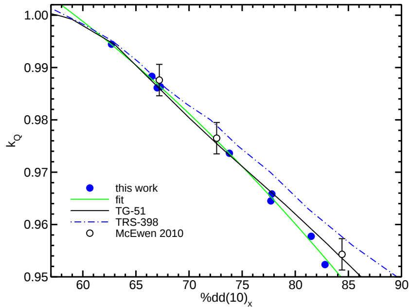
Figure 30: Monte Carlo calculated k_Q factors for the NE2581 ion chamber ( b, 0.6 \text{ cm}^3 ) along with measurements from McEwen, 5 TG-51 6 and TRS-398 values. 7 The fit is to our Monte Carlo values.
