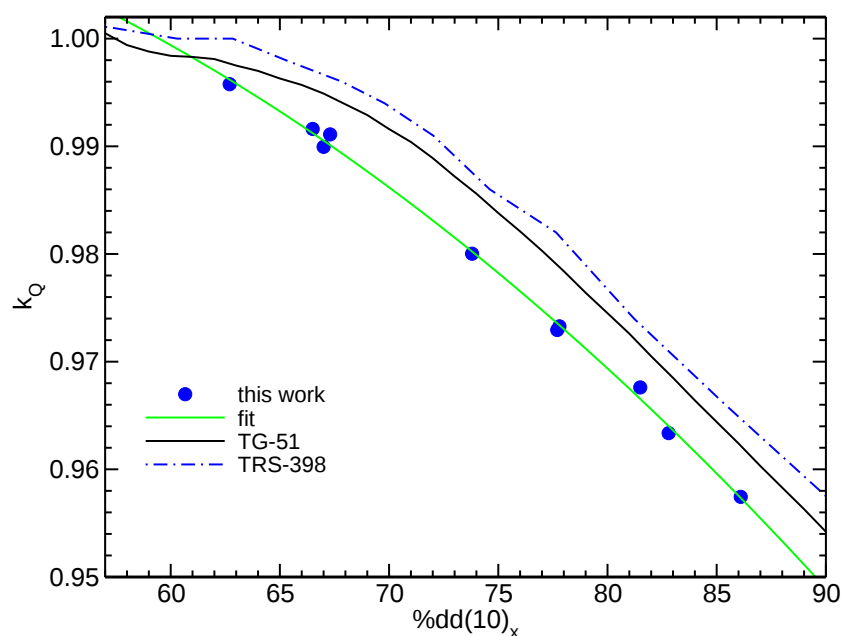
Figure 7: Monte Carlo calculated k_Q factors for the Exradin A1 ion chamber (a, 0.057 cm 3 ) along with TG-51 and TRS-398 values. 6,7 The fit is to our Monte Carlo values.
