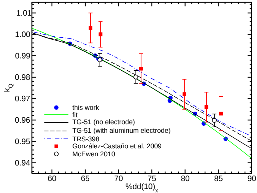
Figure 21: Monte Carlo calculated k_Q factors for the PTW31014 ion chamber ( i, 0.015 \text{ cm}^3 ) along with measurements from McEwen, 5 TG-51 values with and without an aluminum central electrode, 6 TRS-398 values 7 and Monte Carlo data from González-Castaño 8 et al. The fit is to our Monte Carlo values.
