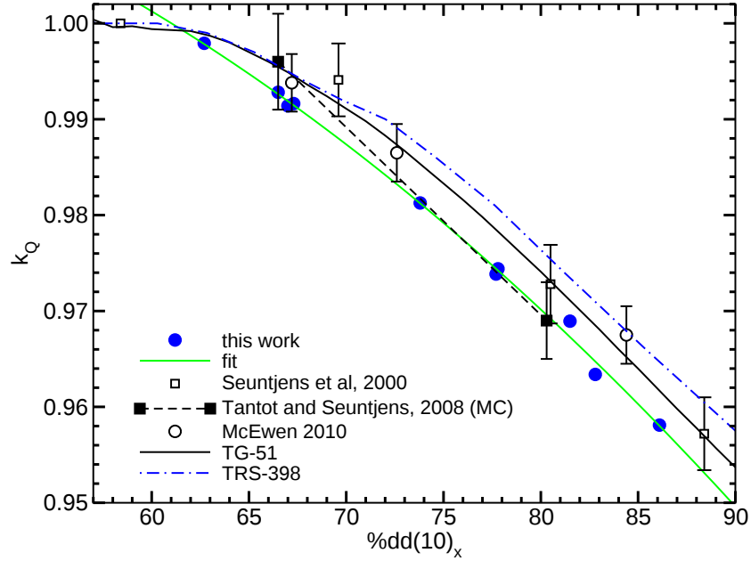
Figure 1: Monte Carlo calculated k_Q factors for the Exradin A12 ion chamber ( a, 0.65 \text{ cm}^3 ) along with measurements, protocol values and Monte Carlo calculations from the literature. 3-7 The fit is to our Monte Carlo values.
