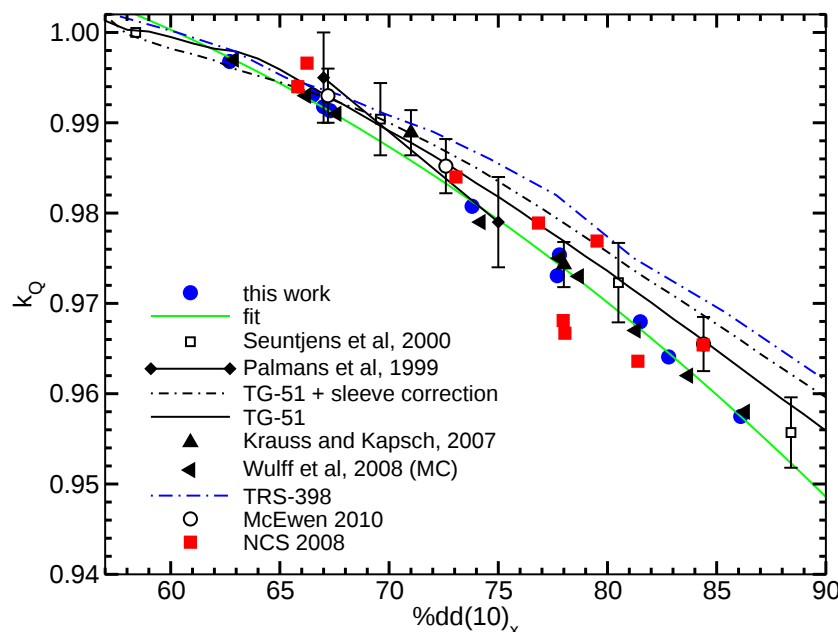
Figure 31: Monte Carlo calculated k_Q factors for NE2571 ion chamber (c,0.6 cm 3 ) along with measurements from McEwen, 5 Seuntjens et al, 3 Krauss and Kapsch 10 and the Netherlands Commission on Radiation Dosimetry Code of Practice, 9 Monte Carlo calculated values from Wulff et al 11 and values from the TG-51 6 and TRS-398 7 protocols. The fit is to our Monte Carlo values.
