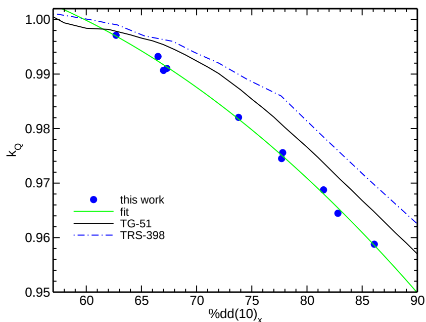
Figure 3: Monte Carlo calculated k_Q factors for the Exradin A2 ion chamber (a, 0.54 cm 3 ) along with TG-51 and TRS-398 values. 6,7 The fit is to our Monte Carlo values.
