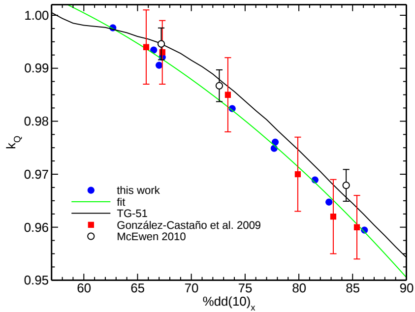
Figure 9: Monte Carlo calculated k_Q factors for the Exradin A1SL ion chamber ( a, 0.057 \text{ cm}^3 ) along with measurements from McEwen, 5 TG-51 values 6 and Monte Carlo data from González-Castaño 8 et al. The fit is to our Monte Carlo values.
