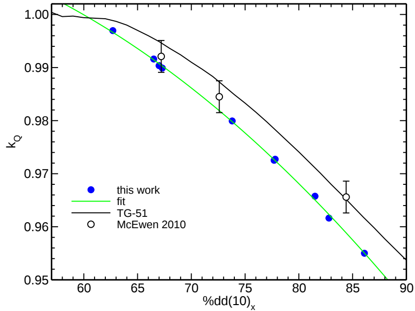
Figure 2: Monte Carlo calculated k_Q factors for the Exradin A19 ion chamber ( a, 0.62 \text{ cm}^3 ) along with measurements from McEwen 5 and TG-51 values. 6 The fit is to our Monte Carlo values.
