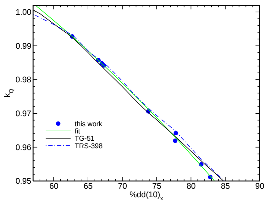
Figure 8: Monte Carlo calculated k_Q factors for the Exradin T1 ion chamber (b, 0.057 cm 3 ) along with TG-51 and TRS-398 values. 6,7 The fit is to our Monte Carlo values.
