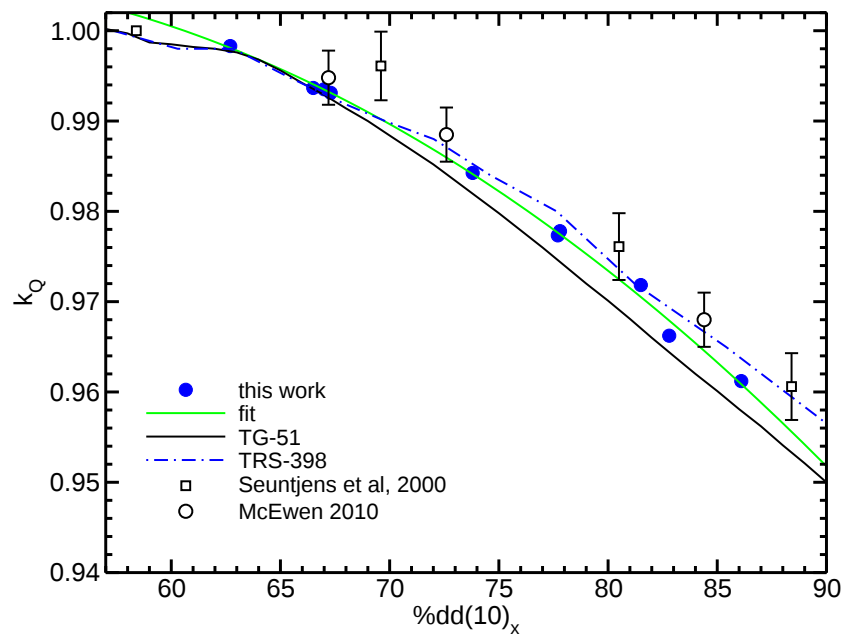
Figure 33: Monte Carlo calculated k_Q factors for the Capintec PR06C/G ion chamber (a,0.65 cm 3 ) along with measurements from McEwen 5 and Seuntjens et al 3 and values from the TG-51 6 and TRS-398 7 protocols. The fit is to our Monte Carlo values.
