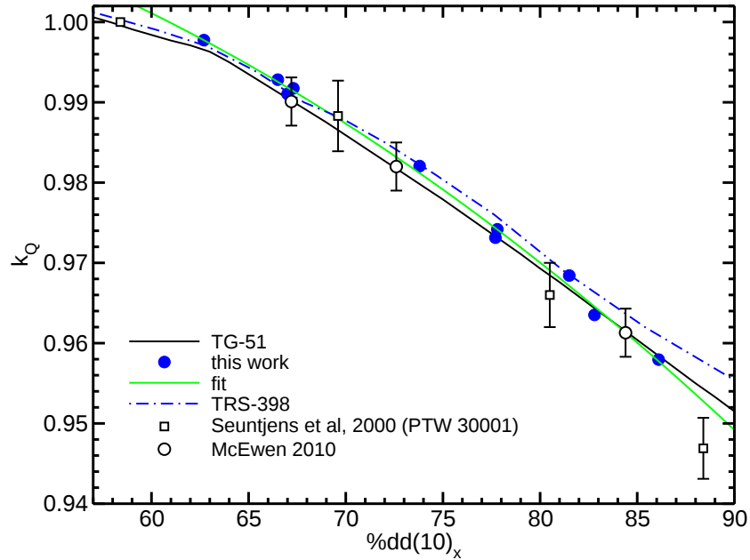
Figure 14: Monte Carlo calculated k_Q factors for the PTW30010 ion chamber ( e, 0.6 \text{ cm}^3 ) along with measurements from McEwen 5 and Seuntjens 3 et al and TRS-398 and TG-51 protocol values. 6,7 The fit is to our Monte Carlo values.
