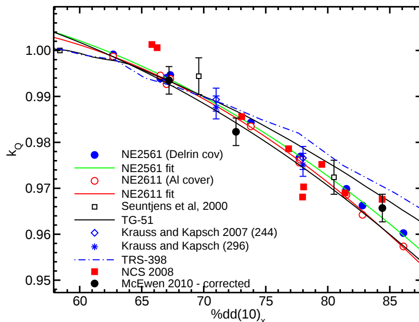
Figure 32: Monte Carlo calculated k_Q factors for the NE2561 and NE2611 ion chambers (c,0.3 cm 3 ) along with measurements from McEwen 5 (corrected, see Muir et al. 12 for details), Seuntjens et al, 3 Krauss and Kapsch 10 and the Netherlands Commission on Radiation Dosimetry Code of Practice 9 and values from the TG-51 6 and TRS-398 7 protocols. The fit is to our Monte Carlo values.
