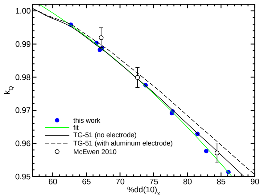
Figure 20: Monte Carlo calculated k_Q factors for the PTW31016 ion chamber ( i, 0.016 \text{ cm}^3 ) along with measurements from McEwen 5 and TG-51 values with and without an aluminum central electrode. 6 The fit is to our Monte Carlo values.
