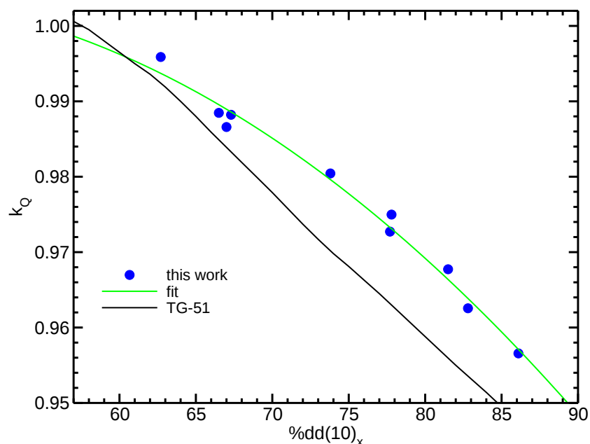
Figure 11: Monte Carlo calculated k_Q factors for the Exradin T14 ion chamber ( h, 0.016 \text{ cm}^3 ) along with TG-51 values. 6 The fit is to our Monte Carlo values.
