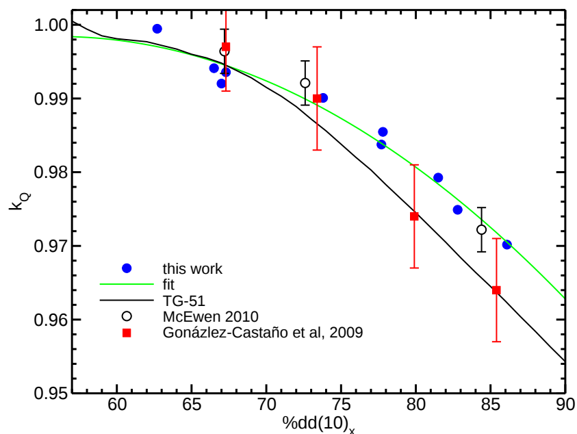
Figure 12: Monte Carlo calculated k_Q factors for the Exradin A14SL ion chamber ( g, 0.016 \text{ cm}^3 ) along with measurements from McEwen, 5 TG-51 values 6 and Monte Carlo data from González-Castaño 8 et al. The fit is to our Monte Carlo values.
