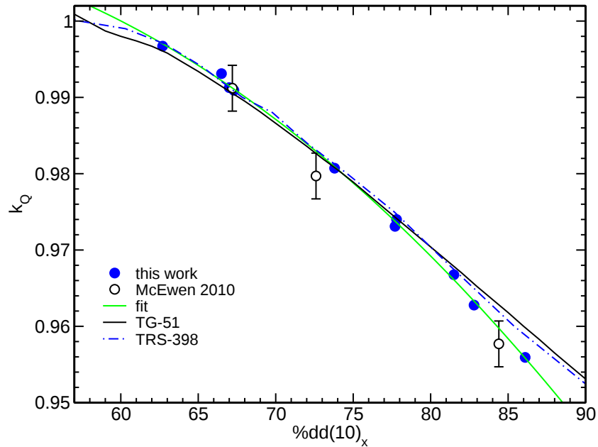
Figure 18: Monte Carlo calculated k_Q factors for the PTW31013 ion chamber ( e, 0.3 \text{ cm}^3 ) along with measurements from McEwen, 5 as well as TRS-398 and TG-51 values. 6,7 The fit is to our Monte Carlo values.
