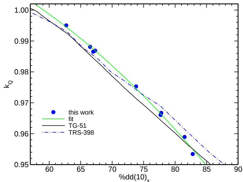
Figure 4: Monte Carlo calculated k_Q factors for the Exradin T2 ion chamber (b, 0.54 cm 3 ) along with TG-51 and TRS-398 values. 6,7 The fit is to our Monte Carlo values.
