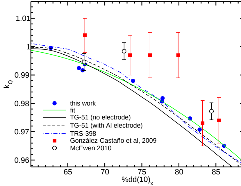
Figure 29: Monte Carlo calculated k_Q factors for the IBA CC01 ion chamber ( g, 0.01 \text{ cm}^3 ) along with measurements from McEwen, 5 TG-51 values with and without an aluminum electrode, 6 TRS-398 values 7 and Monte Carlo data from González-Castaño 8 et al. The fit is to our Monte Carlo values.
