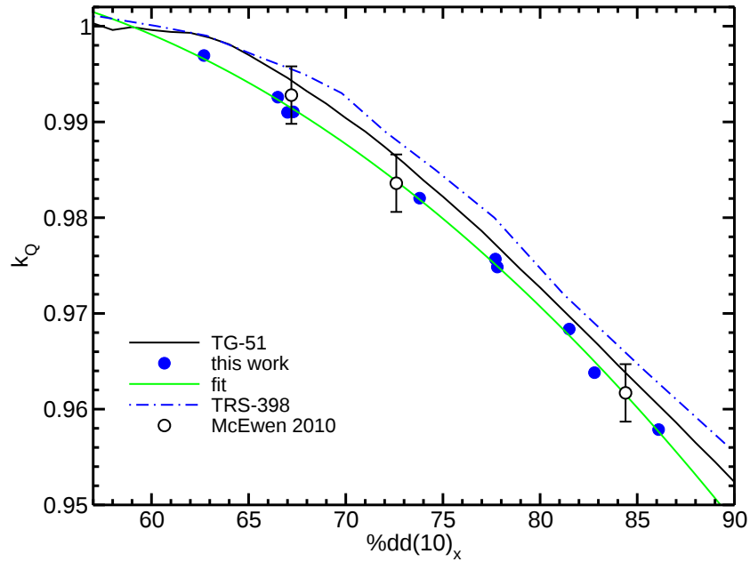
Figure 26: Monte Carlo calculated k_Q factors for the IBA CC13 ion chamber ( a, 0.13 \text{ cm}^3 ) along with measurements from McEwen, 5 TG-51 6 and TRS-398 values. 7 The fit is to our Monte Carlo values.
