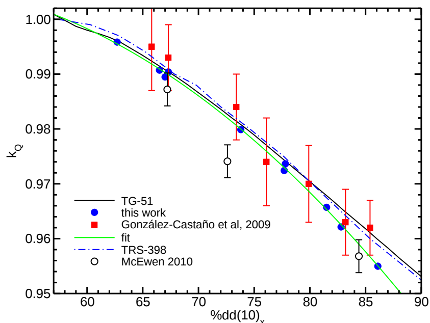
Figure 19: Monte Carlo calculated k_Q factors for the PTW31010 ion chamber ( e, 0.125 \text{ cm}^3 ) along with measurements from McEwen, 5 TRS-398 and TG-51 values 6,7 and Monte Carlo data from González-Castaño 8 et al. The fit is to our Monte Carlo values.
