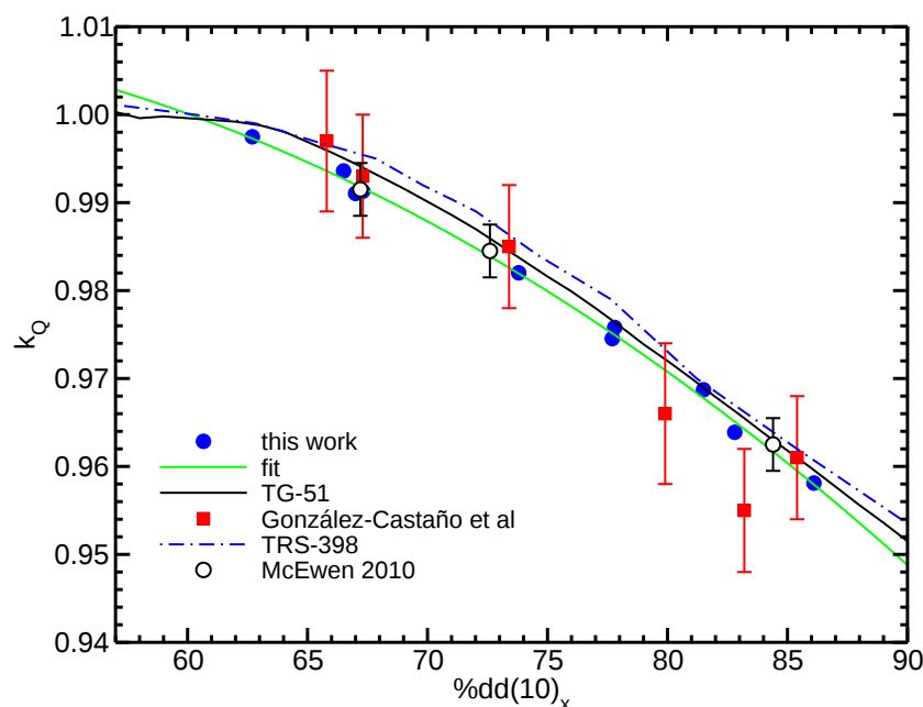
Figure 28: Monte Carlo calculated k_Q factors for the IBA CC04 ion chamber ( a, 0.04 \text{ cm}^3 ) along with measurements from McEwen, 5 TG-51 6 and TRS-398 values 7 and Monte Carlo data from González-Castaño 8 et al. The fit is to our Monte Carlo values.
