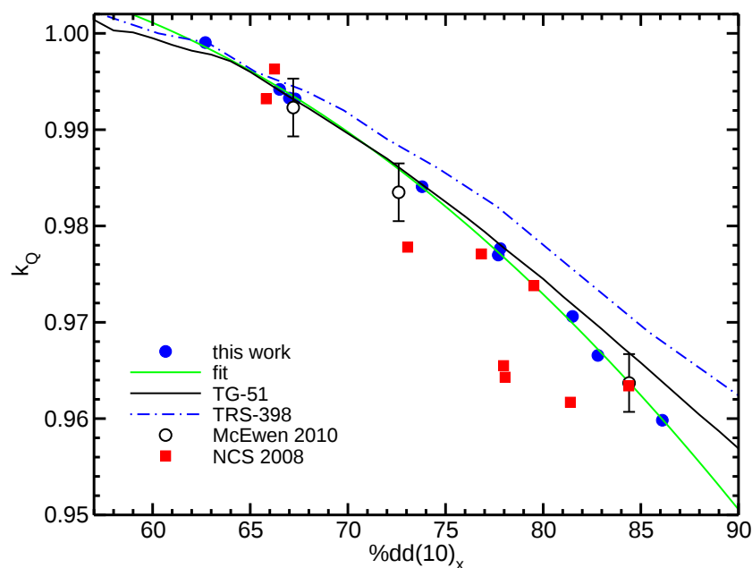
Figure 16: Monte Carlo calculated k_Q factors for the PTW30012 ion chamber ( c, 0.6 \text{ cm}^3 ) along with measurements from McEwen, 5 TRS-398 and TG-51 values 6,7 and values measured for the Netherlands Commission on Radiation Dosimetry Code of Practice. 9 The fit is to our Monte Carlo values.
