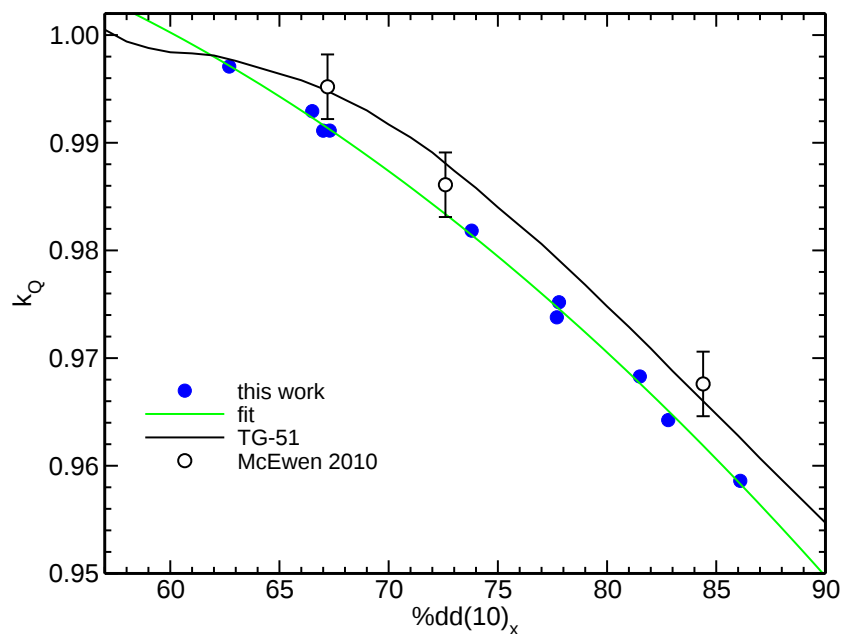
Figure 6: Monte Carlo calculated k_Q factors for the Exradin A18 ion chamber ( a, 0.125 \text{ cm}^3 ) along with measurements from McEwen 5 and TG-51 values. 6 The fit is to our Monte Carlo values.
