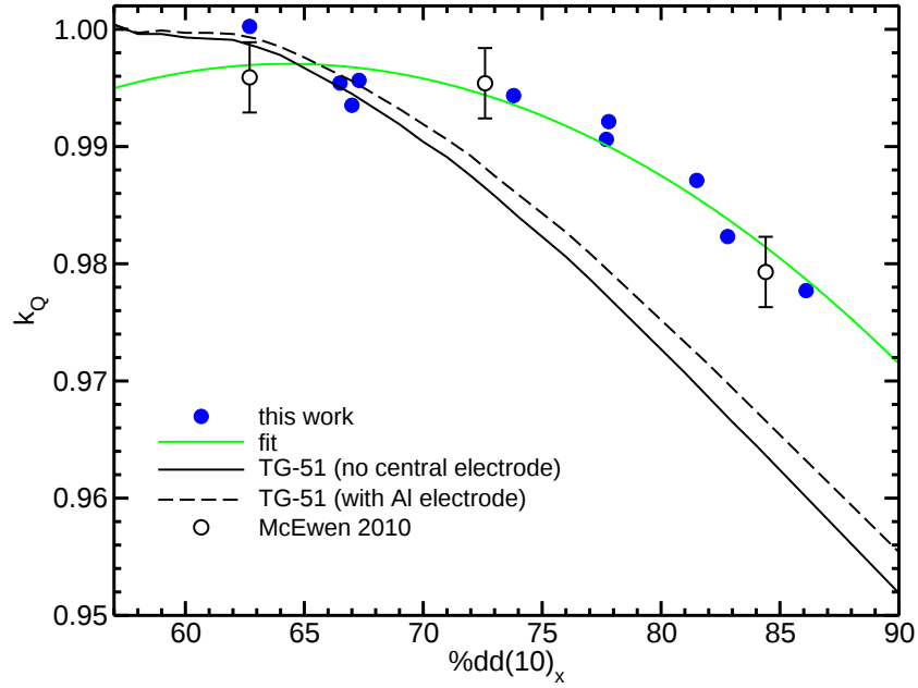
Figure 13: Monte Carlo calculated k_Q factors for the Exradin A16 ion chamber ( g, 0.007 \text{ cm}^3 ) along with measurements from McEwen 5 and TG-51 values with and without an aluminum electrode. 6 The fit is to our Monte Carlo values.
