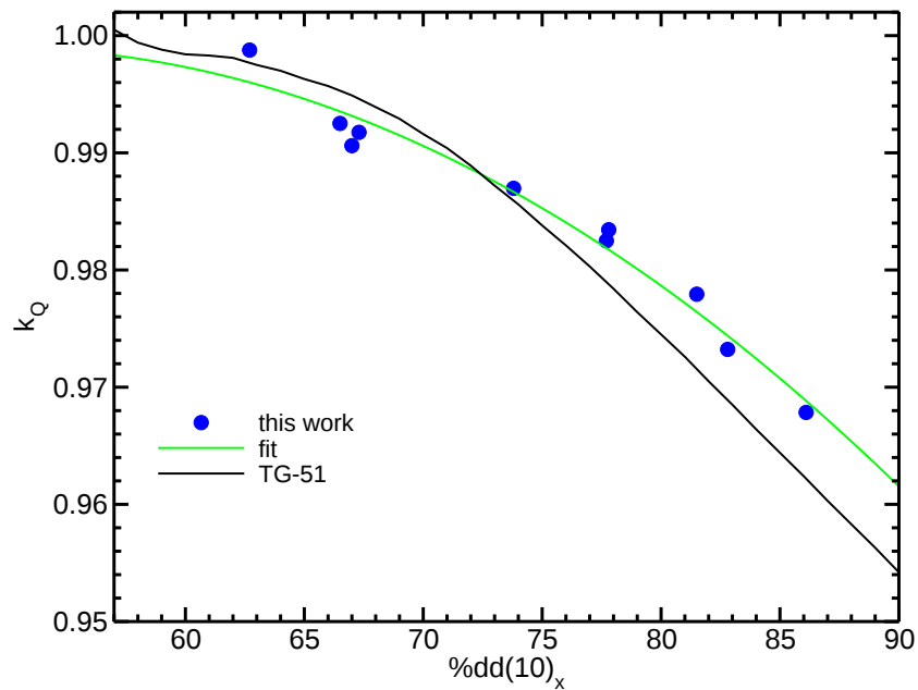
Figure 10: Monte Carlo calculated k_Q factors for the Exradin A14 ion chamber ( g, 0.016 \text{ cm}^3 ) along with TG-51 values. 6 The fit is to our Monte Carlo values.
