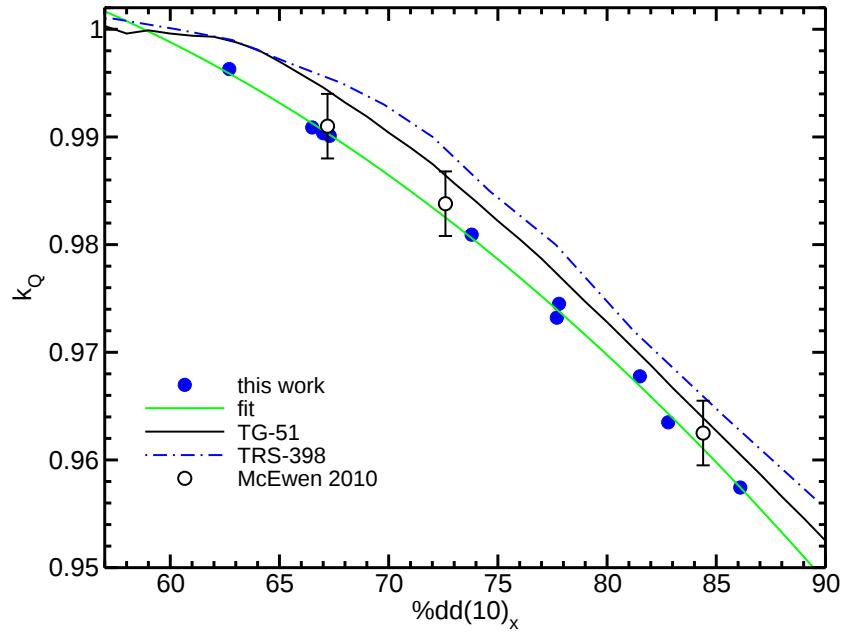
Figure 25: Monte Carlo calculated k_Q factors for the IBA FC23C ion chamber ( a, 0.23 \text{ cm}^3 ) along with measurements from McEwen, 5 TG-51 6 and TRS-398 values. 7 The fit is to our Monte Carlo values.
