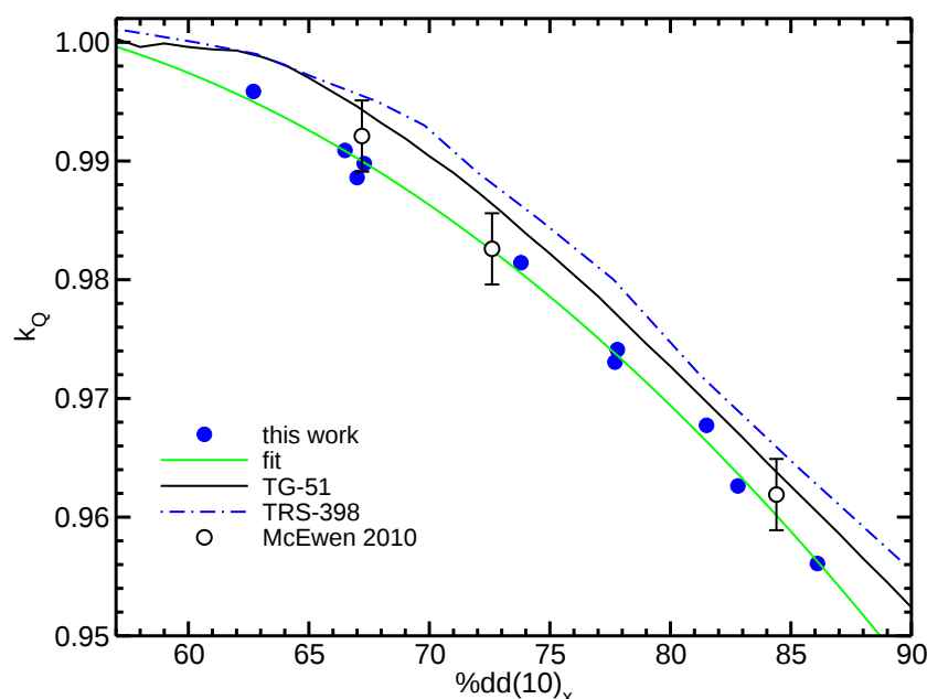
Figure 27: Monte Carlo calculated k_Q factors for the IBA CC08 ion chamber ( a, 0.08 \text{ cm}^3 ) along with measurements from McEwen, 5 TG-51 6 and TRS-398 values. 7 The fit is to our Monte Carlo values.
